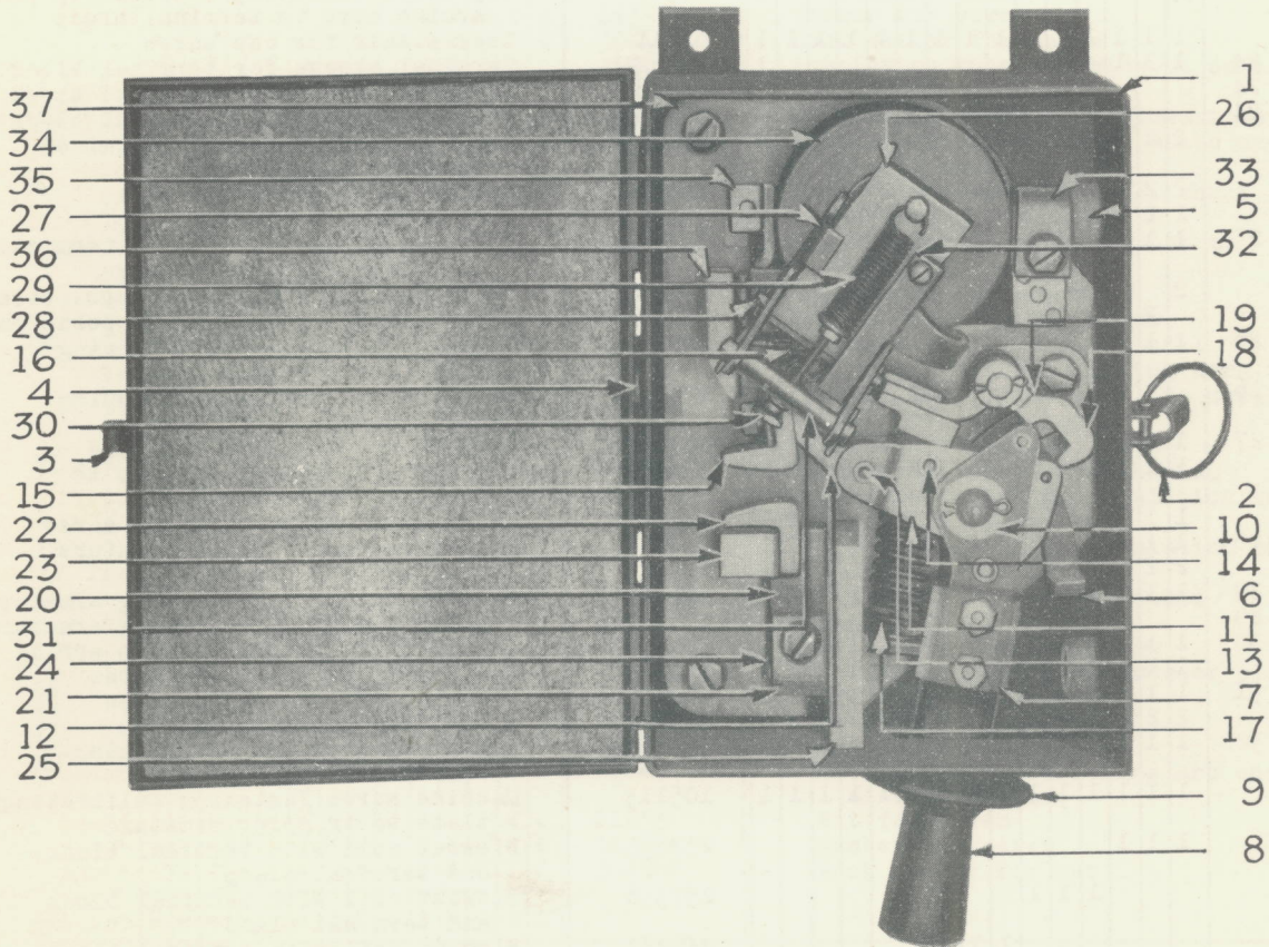
TYPE MR-21 FORM A AUTOMATIC CIRCUIT BREAKER
